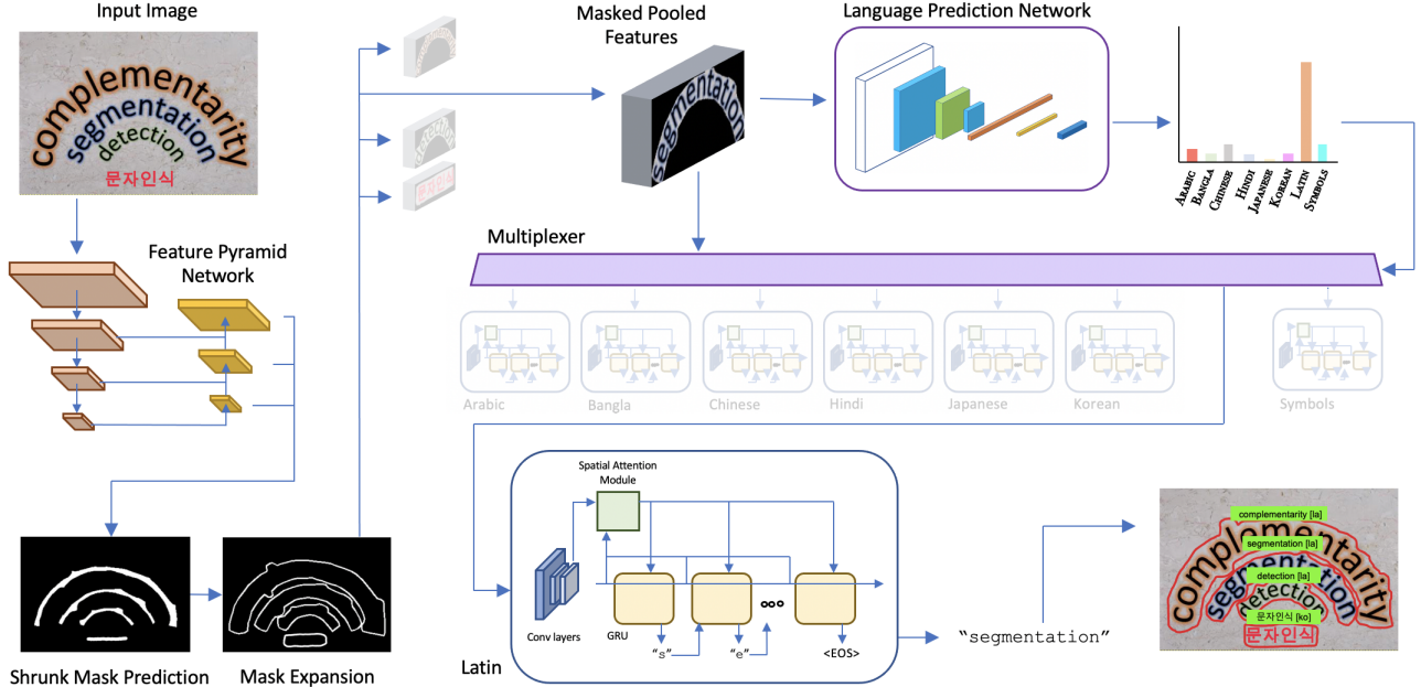
Figure 1. M3 TextSpotter . The proposed M3 TextSpotter shares the same detection and segmentation trunk with Mask TextSpotter v3 [30], but incorporates a novel Language Prediction Network (LPN). The output of the LPN then determines which script’s recognition head the multiplexer selects.
